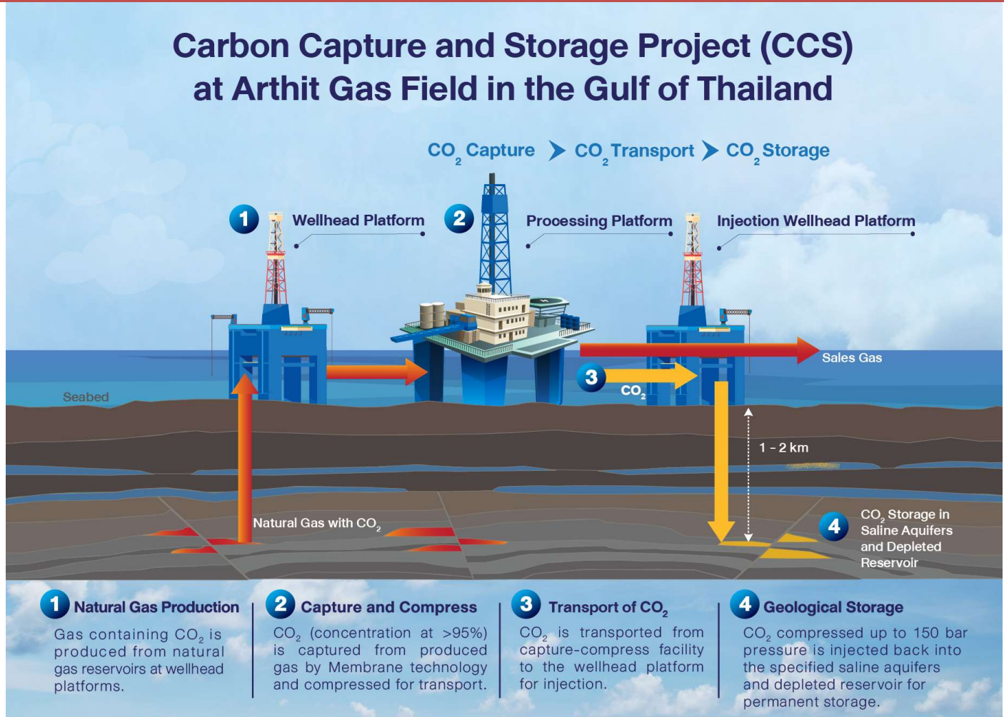
Fig 1.: PTTEP CCS at Arthit Field
